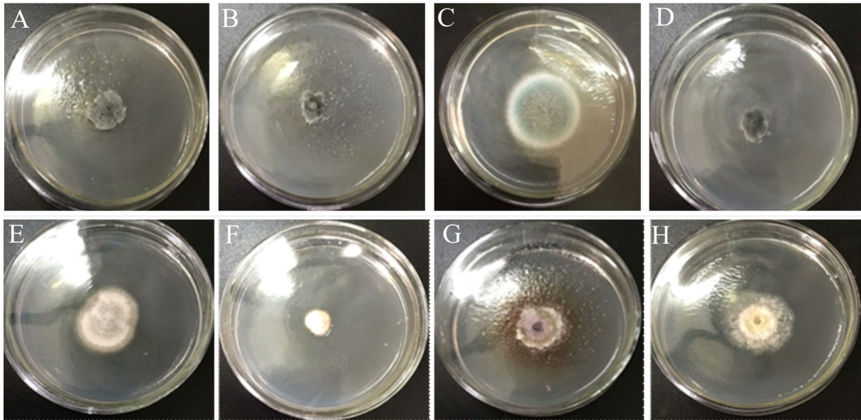
A. 菌株 ye-130; B. 菌株 ye-134; C. 菌株 ye-135; D. 菌株 ye-136; E. 菌株 jing-116; F. 菌株 jing-117; G. 菌株 jing-119; H. 菌株 jing-180。 A. Strain ye-130; B. Strain ye-134; C. Strain ye-135; D. Strain ye-136; E. Strain jing-116; F. Strain jing-117; G. Strain jing-119; H. Strain jing-180.
