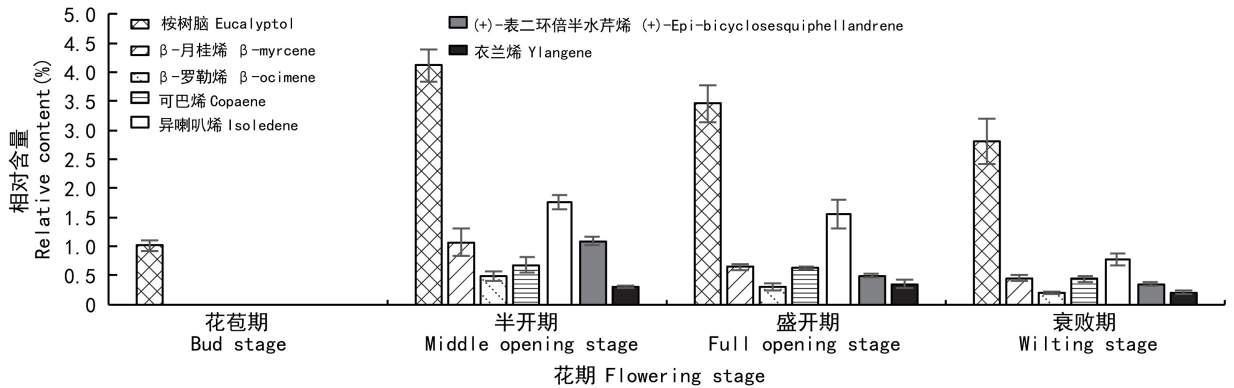
图 4 第 1 主成分高度正相关萜烯类物质不同花期相对含量的变化 Fig. 4 Changes of relative content of different flowering stages of terpenoids with highly positive correlation of the first principal component
