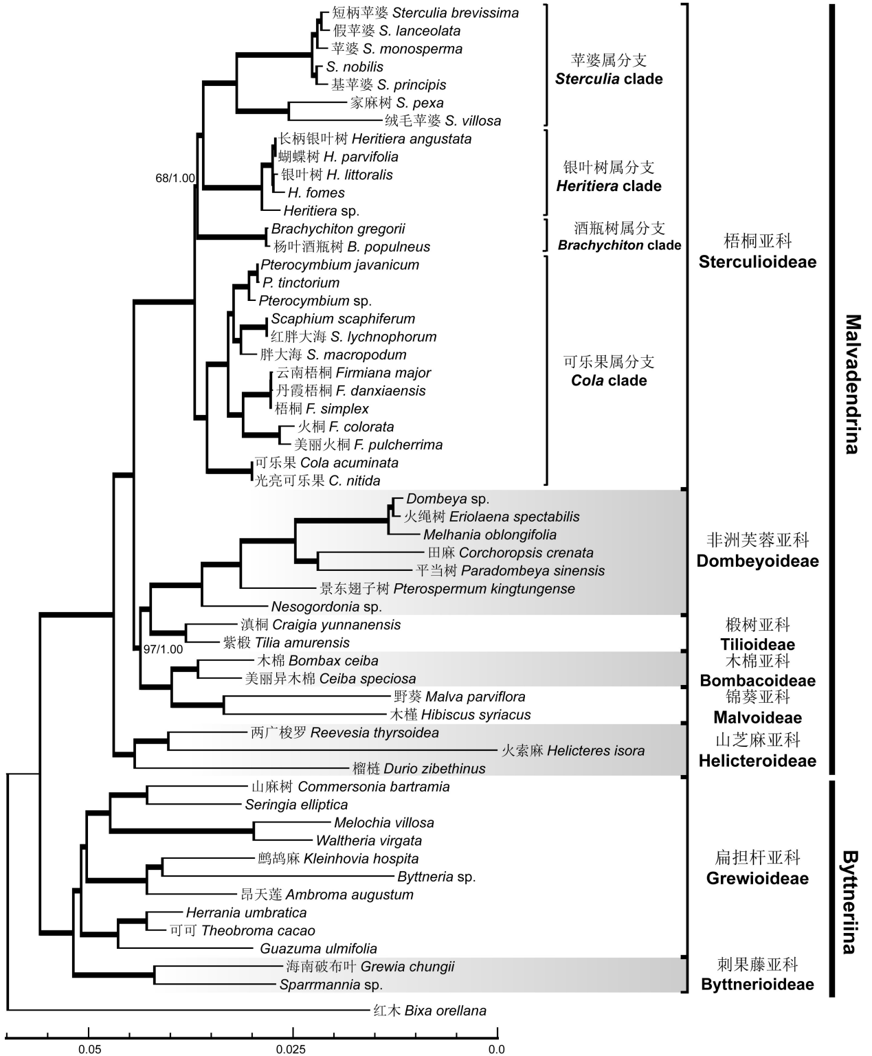
仅显示主要节点支持率。数字表示分支的最大似然的 bootstrap 值/贝叶斯后验概率。未标注的分支支持率为 100%/1.0。 Only major node support value is shown. The labels indicate maximum likelihood bootstrap support/Bayesian posterior probabilities. Unlabeled branches have 100%/1.0 support values.
