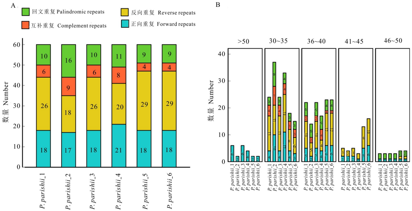
A. 不同类型重复序列的数量；B. 重复序列的类型在不同重复长度中的数量分布。 A. Numbers of repeat sequences in different types; B. Frequency distributions of different types of repeat sequences identified in different sizes of the chloroplast.
