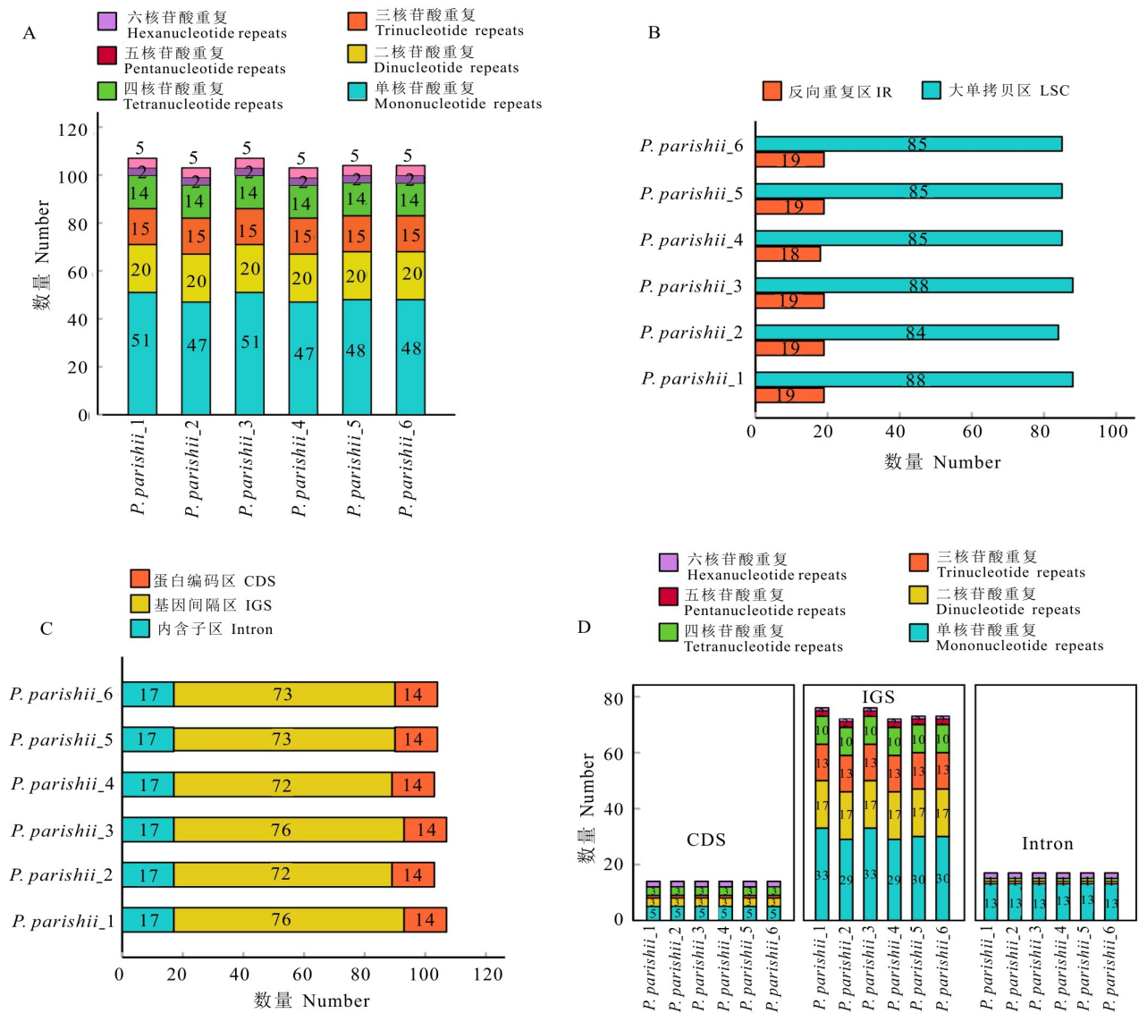
A. 不同类型重复单元的数量; B. SSR 位点在叶绿体基因组大单拷贝区 (LSC)、小单拷贝区 (SSC) 和反向重复区 (IR) 的数量; C. SSR 位点在 CDS、IGS、Intron 区域的数量; D. SSR 位点分别在叶绿体基因组 CDS、IGS、Intron 区域不同重复类型的数量分布。 A. Numbers of SSRs in different types; B. Numbers of SSRs in the LSC, SSC, and IR regions; C. Numbers of SSRs identified in CDS, IGS, and introns of the cp genome; D. Frequency distribution of different types of SSRs identified in CDS, IGS, and introns of the cp genome.
