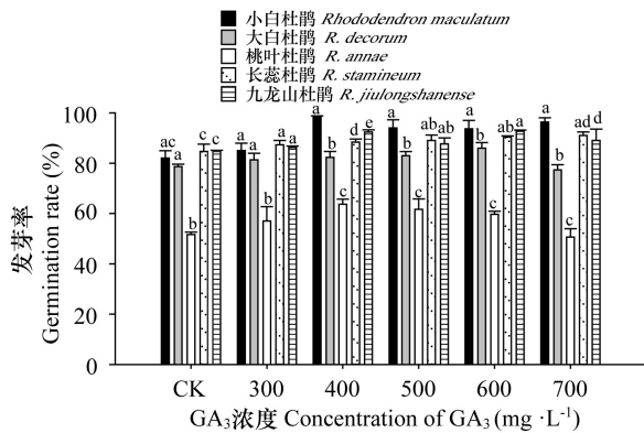
图 1 不同浓度 GA 3 处理下五种晚花杜鹃种子发芽率比较 Fig. 1 Comparison of germination rate of five species of late flower Rhododendron with different concentrations of GA 3
