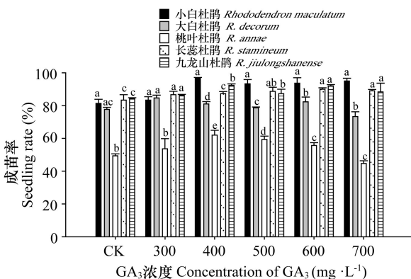
图 2 不同浓度 GA 3 处理下五种晚花杜鹃种子成苗率比较 Fig. 2 Comparison of seedling rate of five species of late flower Rhododendron with different concentrations of GA 3
